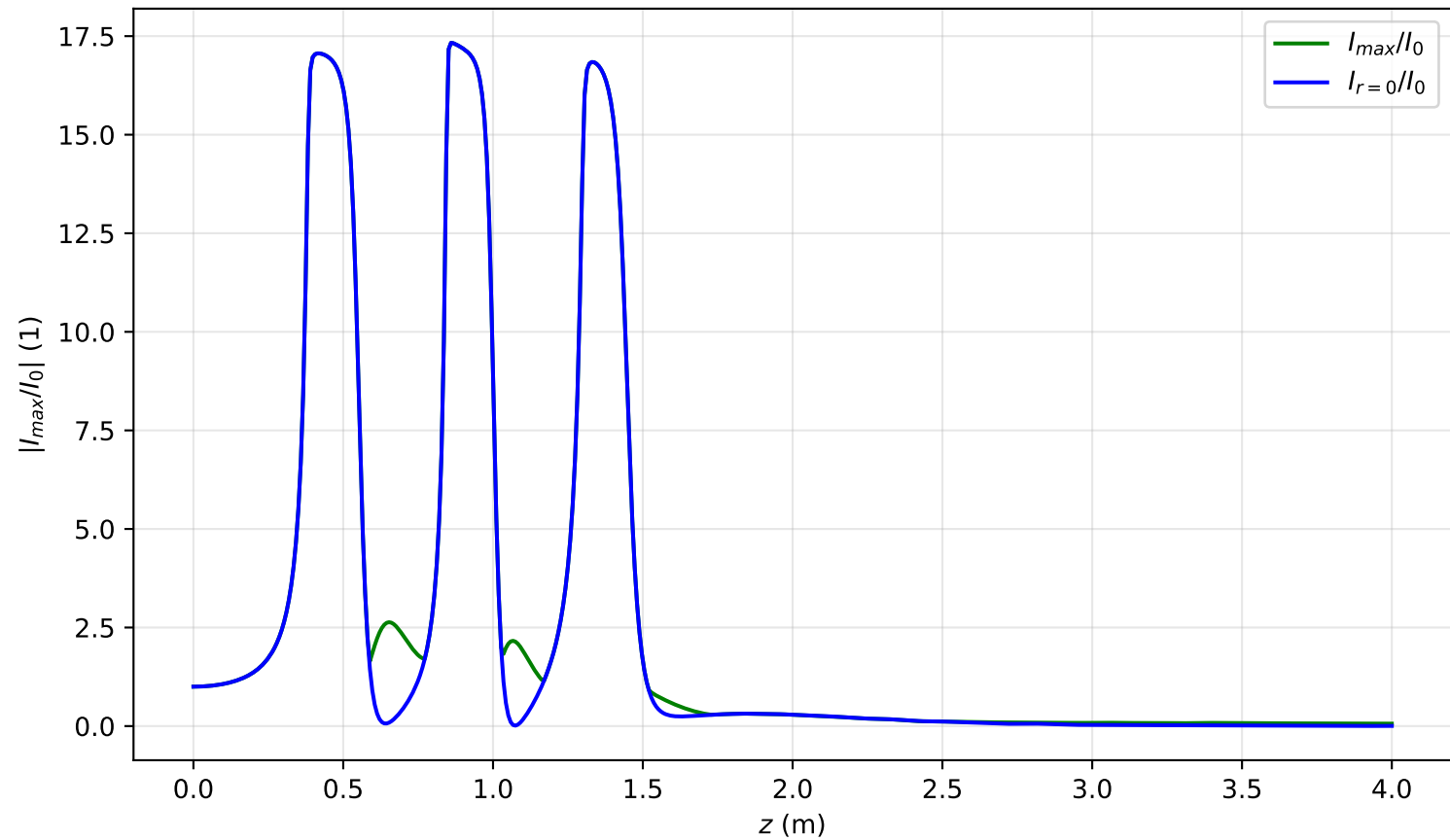
I_{max}(x = 0, y = 0, z)/I_0 , Pin=6.5Pcr, artificial time
